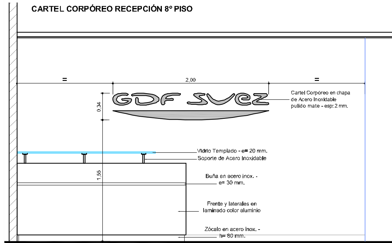
VISTA FRONTAL
