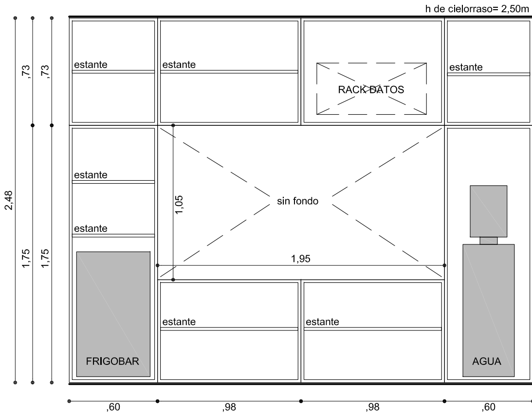
VISTA INTERIOR
