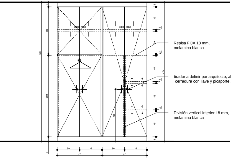
VISTA FRONTAL
