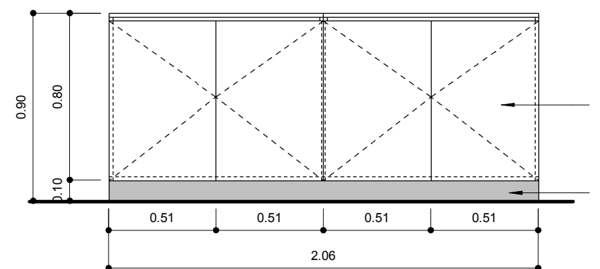
VISTA FRONTAL
