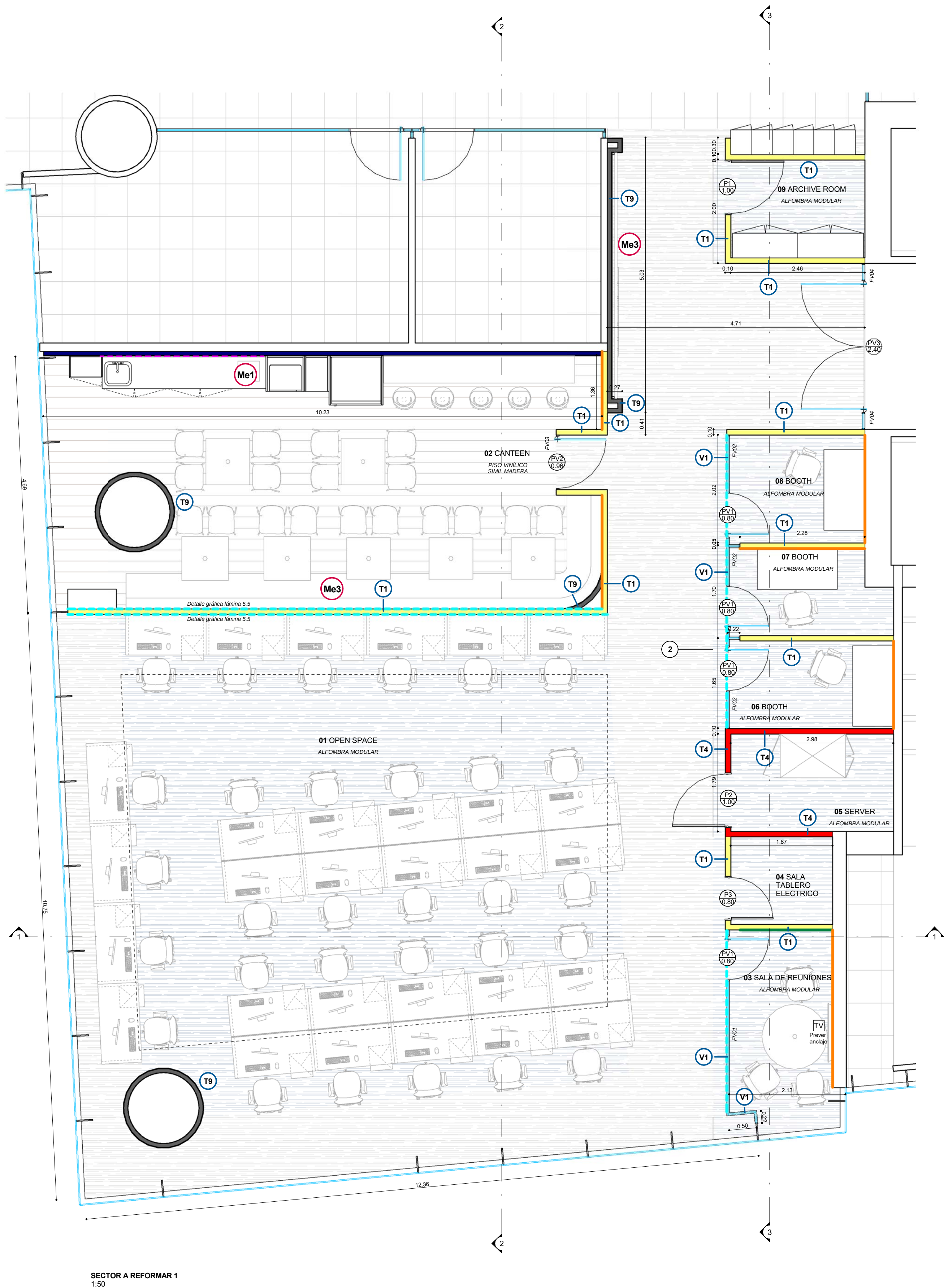
SECTOR A REFORMAR 1 1:50
