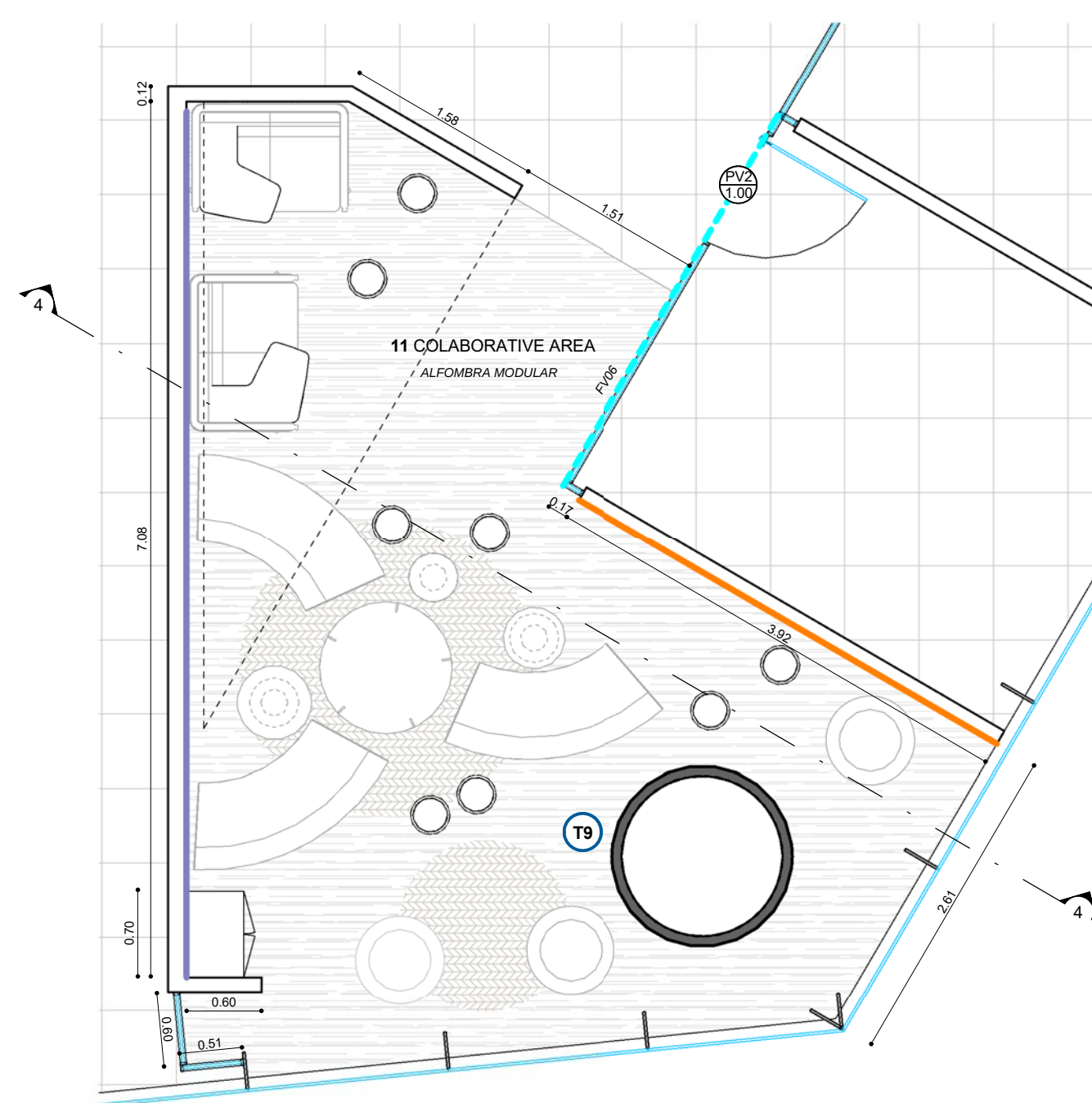
SECTOR A REFORMAR 3 1:50
