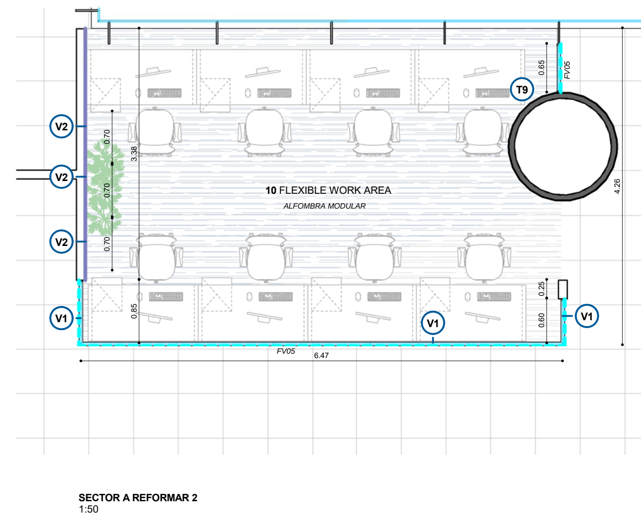
SECTOR A REFORMAR 2 1:50
